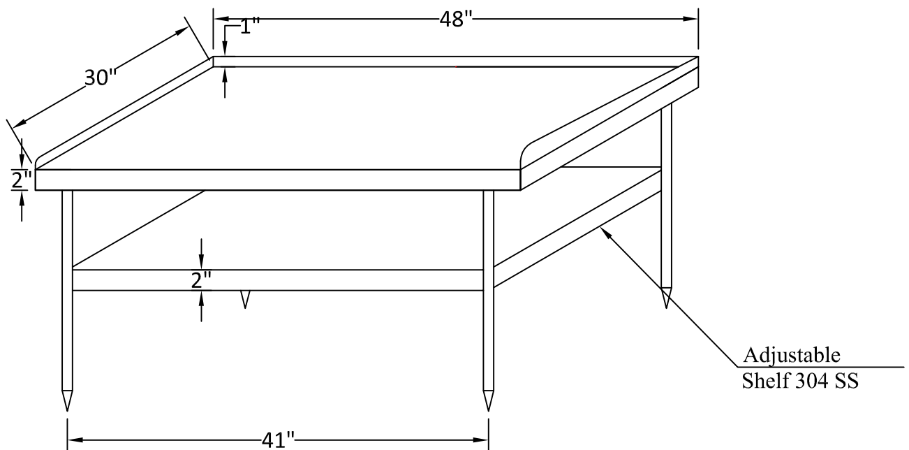
48" Equipment Table Model: WE-ET1
